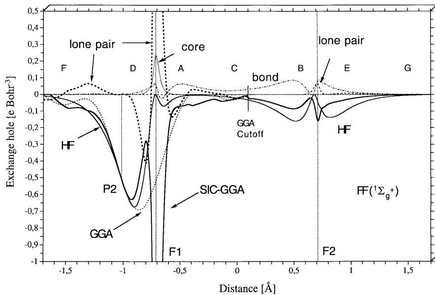
Fig. 7. Graphical representation of the exchange hole calculated for F_2 ( ^1\Sigma_g^+ ) along the bond axis at the HF ( solid line ), GGA ( dashed line ), and SIC-GGA ( bold line ) levels of theory for the reference point being at position P2. The core, lone pair, and bond orbital contributions to the SIE of the GGA exchange functional are given by dashed lines . All calculations with a cc-pVTZ basis set at the experimental geometry
