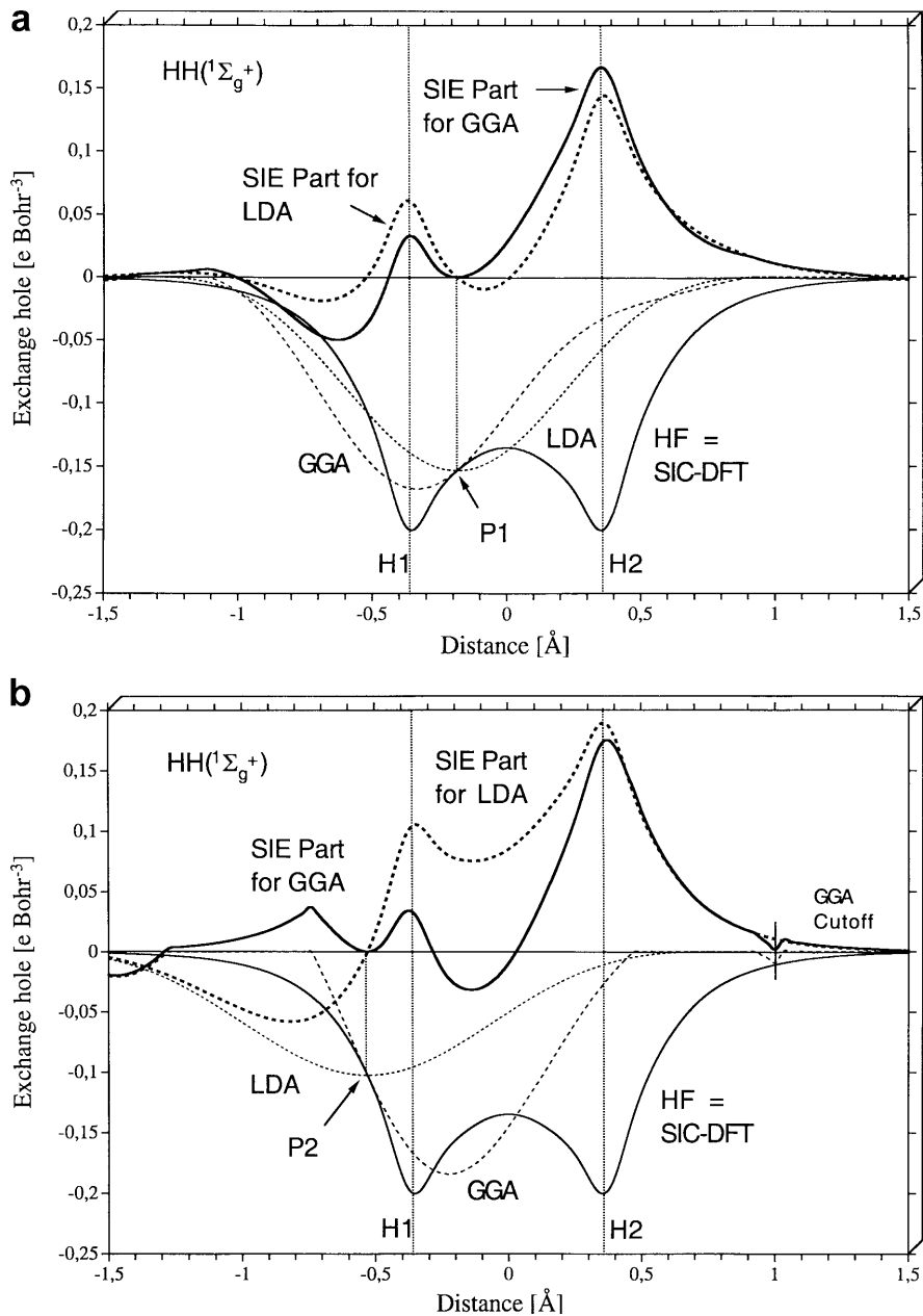
Fig. 1. Graphical representation of the exchange hole calculated for \text{H}_2 ( ^1\Sigma_g^+ ) along the bond axis at the Hartree-Fock (HF) (solid line), local density approximation (LDA) (short-dashed line) and, generalized gradient approximation (GGA) (long-dashed line) levels of theory for the reference electron being a at position P1 and b at position P2. The self-interaction-error (SIE) parts of the GGA and LDA hole are indicated in bold and bold-dashed print, respectively. All calculations with a cc-pVTZ basis set at the experimental H-H distance
